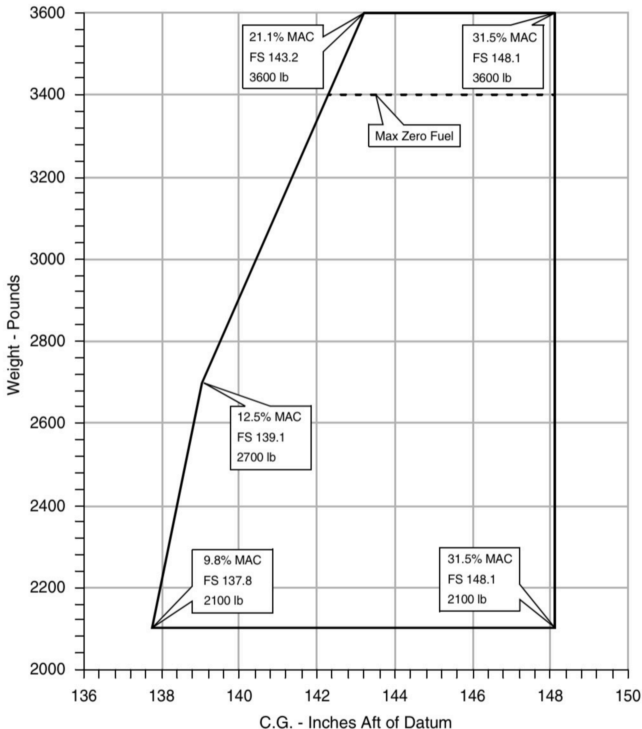
Figure 2-1: Center of Gravity Envelope
